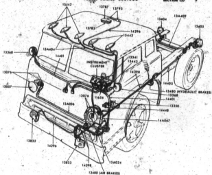
WIRING SYSTEM-INTERIOR AND EXTERIOR LAMPS 1973/ C-CT600/900
