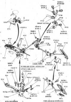
ACCELERATOR and TRANSMISSION LINKAGE 1974/79 B-600-6 CYL. 300
