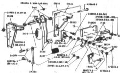
-BRAKE PEDAL and LINKAGE PARTS (SPLIT HYDRAULIC BRAKE) 1973 / C-CT600/900
