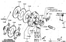
CLUTCH ASSY. (14" DUAL PLATE)
