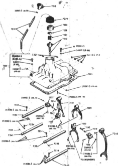
GEARSHIFT MECHANISM (5 SPEED)-NEW PROCESS 542-TYPICAL 1973/ B-F600/750
