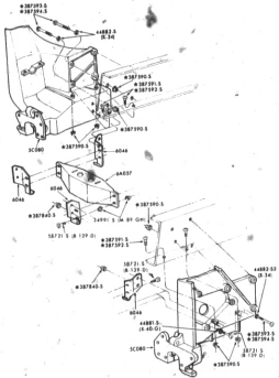
ENGINE SUPPORT-w/FRAME EXTENSION BRACKET (FRONT) 1970/ CL-CL1900
