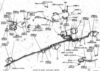
AIR BRAKE SYSTEM (BRAKE SKID CONTROL-REAR SECTION) 1975/ CT800/900
